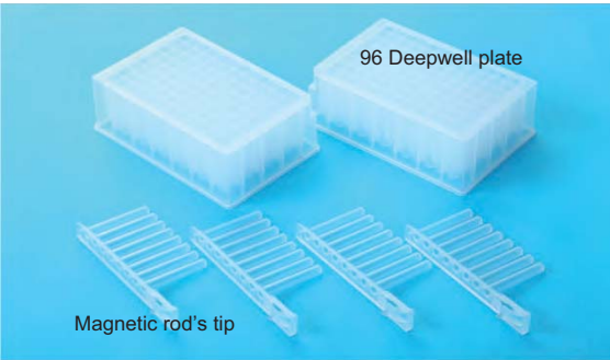
Auto-Pure16A consumable
